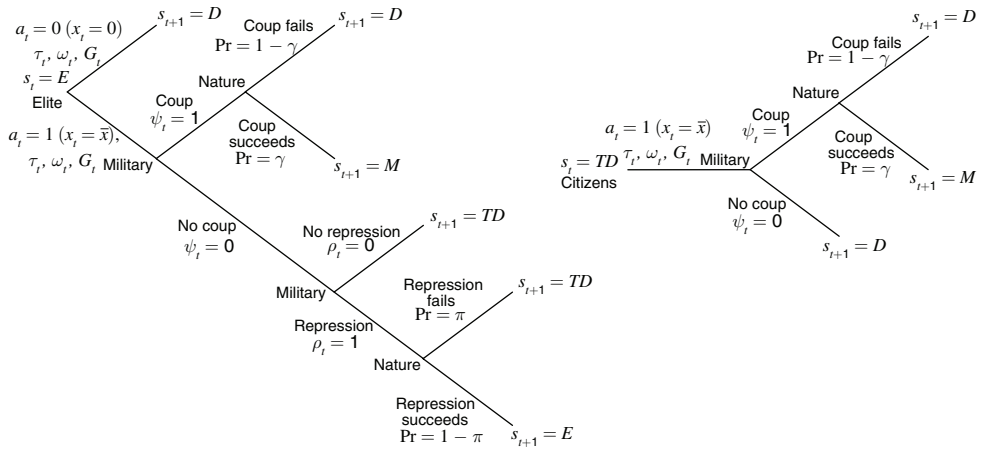
FIGURE 1. THE GAME FORMS STARTING FROM OLIGARCHY ( s_t = E ) AND TRANSITIONAL DEMOCRACY ( s_t = TD )
