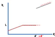
(a) An increase in fine, \phi ; externality, \hat{\phi}_{inc} ; or public enforcement, \eta .
